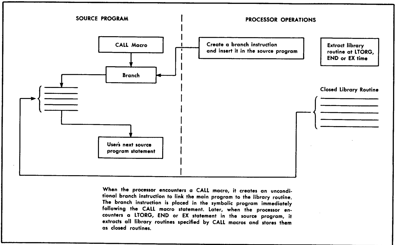
Figure 77. CALL Processing
