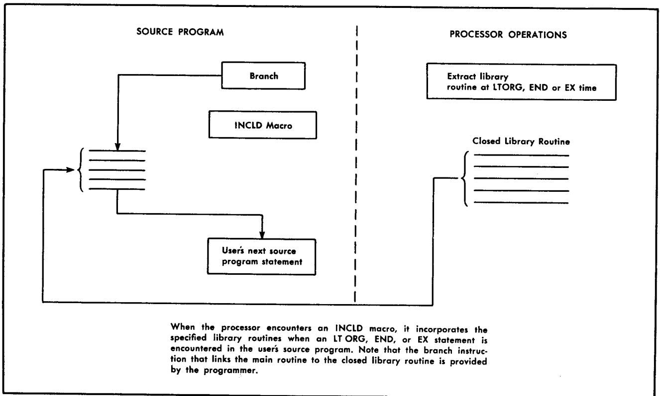
Figure 78. INCLD Processing
